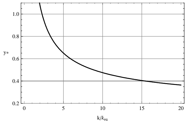
FIG. 3: The time at which the contribution of the cold dark matter and of the radiation are comparable in the Poisson equation as a function of k/k_{\text{eq}} . k_{\text{eq}} is the wave-number of the mode that becomes sub-Hubble at the time of equality. For most of the scales of interest, i.e. for k \gg k_{\text{eq}} , the contribution of the CDM in the Poisson equation is dominant before equality, i.e. y_* < 1 ).
