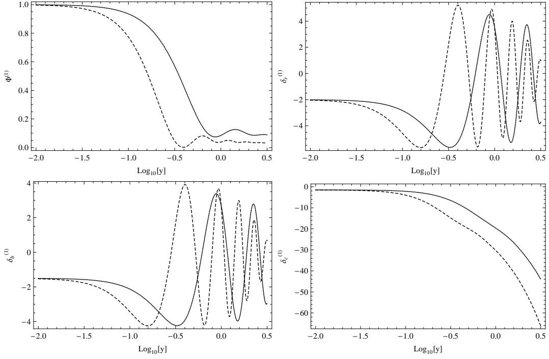
FIG. 7: From top to bottom, left to right: evolution of the Bardeen potential, \Phi , and the density contrast \delta for respectively the radiation, the baryons and the cold dark matter. The solid line corresponds to k = 10k_{\text{eq}} and the dashed line corresponds to k = 20k_{\text{eq}} .
