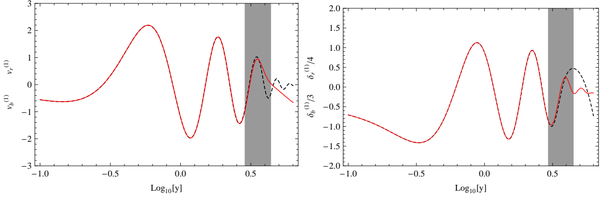
FIG. 8: Left: Comparison of the baryon and photon velocity perturbation at first order for k = 10k_{\text{eq}} . It shows that v_r^{(1)} = v_b^{(1)} with a good approximation until decoupling. Right: Comparison of \frac{1}{4}\delta_r^{(1)} and \frac{1}{3}\delta_b^{(1)} . It can be seen that the adiabaticity condition holds until recombination, hence justifying the approximation of § III.
