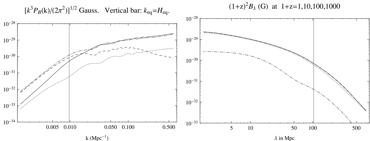
FIG. 1: Left: Magnetic field spectrum today (solid). Contributions from the different sources in (5) are distinguished: second order velocity term S_1 (dot-dashed), quadratic term S_2 in velocity and density (dashed), quadratic term S_3 in anisotropic stress and velocity (dotted). Right: Comoving magnetic field strength at a given scale at times 1+z=1, 10, 100, 1000 corresponding respectively to solid, dashed, dotted and dot-dashed lines. (Dashed and solid lines cannot be distinguished).
