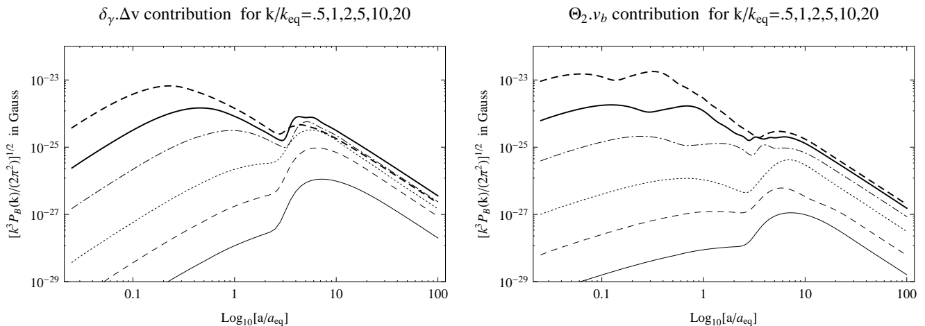
FIG. 3: Left : Magnetic field spectrum P_B^{S_2}(k, \eta) from only the S_2 contribution in (57), for different k/k_{\text{eq}} , with values increasing from bottom to top. Right : Magnetic field spectrum P_B^{S_3}(k, \eta) from only the S_3 contribution in (57).
