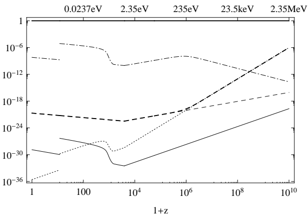
FIG. 2: Evolution with redshift of different ratios between characteristic times that arise in (31), compared with unity (thick black line): \eta_C \tau_C / (\tau_{\text{evo}}^2) (thin solid), \eta_C / \tau_{\text{evo}} (thin dashed), \eta_C \tau_C / (\tau_{\text{evo}} \tau_T) (dotted), \eta_C \tau_C / (\eta_{C,\text{eff}} \tau_{\text{evo}}) (dot-dashed) and \eta_{C,\text{eff}} / \tau_{\text{evo}} (thick dashed).
