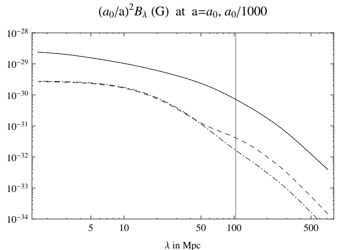
FIG. 5: Magnetic field strength at a given scale as measured in the fundamental frame at 1+z = 1 (continuous) and 1+z = 1000 (dashed), and as measured in the baryon frame at 1+z = 1 (dotted) and 1+z = 1000 (dot-dashed). Dotted and continuous lines cannot be distinguished.
