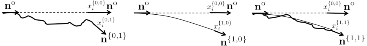
FIG. 1: Comparison of the geodesic in the approximation at order \{n, p\} . In order to adopt an observer based point of view, we need to relate the local direction of propagation \mathbf{n}^{\{n,p\}} to \mathbf{n}^o . The transports for the 3 orders of perturbations are respectively detailed in Eqs. (6.12) and (6.37) that determine x^{i\{n,p\}}(\chi, \mathbf{n}^o) that can be further split in a radial component \delta r^{\{n,p\}}(\chi, \mathbf{n}^o) and an orthoradial contribution that defines the deflection angle \alpha^{a\{n,p\}}(\chi, \mathbf{n}^o) .
