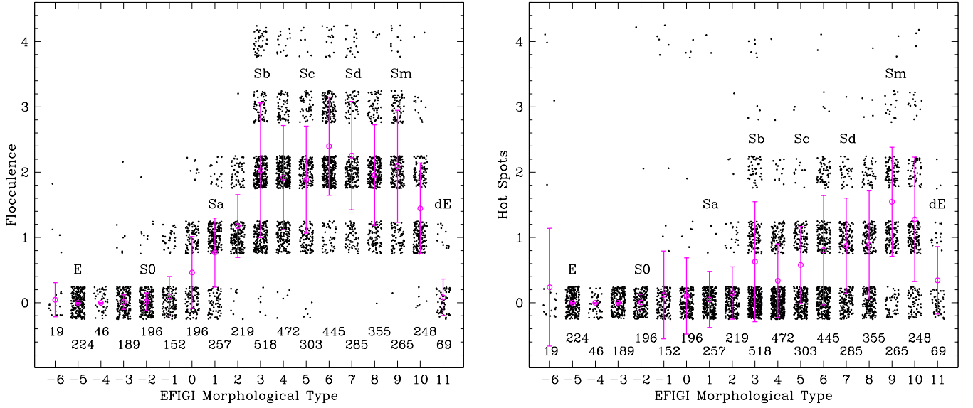
Fig. 15. Same as Fig. 7 for the Flocculence (left) and Hot Spots (right) attributes. The left panel shows the nearly constant level of Flocculence for all spiral types Sb and later and the lower values for Sa and Im galaxies. The right panel shows a nearly constant level of Hot Spots for all spiral types from Sb to Sdm and an increased Hot Spots attribute for Sm and Im types.
