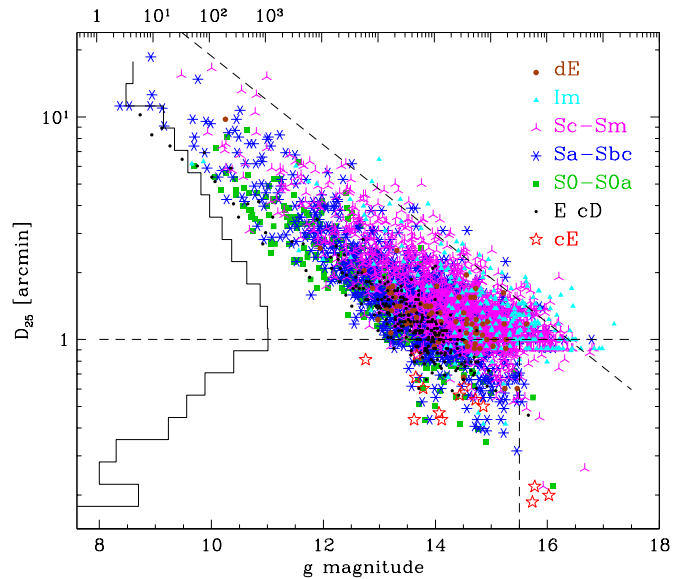
Fig. 3. Distribution of apparent major isophotal diameter D_{25} converted into arcminutes as a function of g -magnitudes measured (de Lapparent & Bertin 2011a) for the 4204 EFIGI galaxies for which these parameters are defined. Different symbols and colours are used for different EM-types. The histogram of D_{25} in intervals of 0.1 arcminutes, overplotted vertically on a log scale and with corresponding labels on the top axis of the graph, demonstrates the strong incompleteness in the catalogue for D_{25} < 1' and B_T > 15.5 , materialised by the horizontal and vertical dashed lines. The diagonal dashed line corresponds to a surface brightness limit of 25 mag/arcsec 2 . The EFIGI catalogue is most complete between these diameter and surface brightness limits, and the crossing of these two lines causes the disappearance of data points fainter than g \sim 16.5 .
