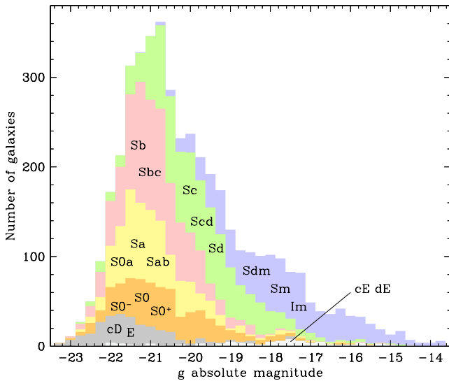
Fig. 2. Absolute magnitude distribution in the g -band for all EFIGI galaxies separated by EFIGI morphological type, grouped as follows: cE-dE (light grey) ; E-cD (grey); S0 - -S0-S0 + (orange); S0a-Sa-Sab (yellow); Sb-Sbc (pink); Sc-Scd-Sd (green); Sdm-Sm-Im (blue).
