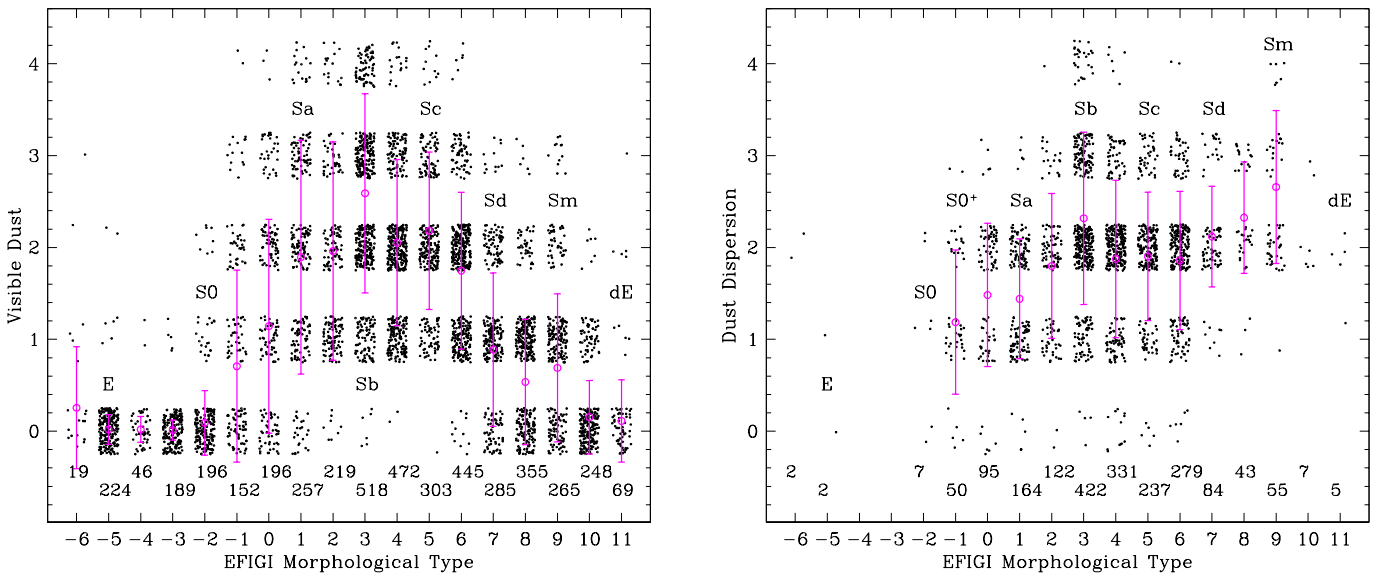
Fig. 14. Distribution of the Visible Dust (left) and Dust Dispersion (right) attributes for the 4458 and 1905 EFIGI galaxies for which these attributes are defined (same presentation as in Fig. 5). The left panel shows the large amounts of dust for early and intermediate spiral types (Sa to Scd), with a peak for Sb galaxies, and the lower values for late spiral (Sd to Sm) and Im types. The right panel shows the increasing Dust Dispersion for spiral galaxies of later type.
