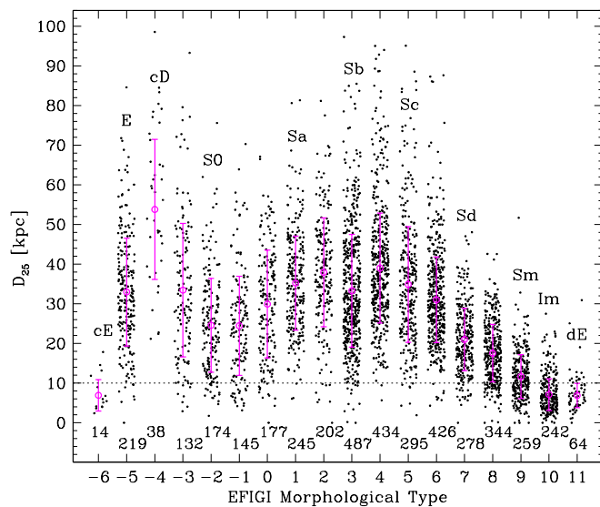
Fig. 16. Distribution of intrinsic isophotal diameter in kpc for 4196 EFIGI galaxies as a function of EFIGI morphological type. For each type, the weighted mean and r.m.s. dispersion (with 3-sigma clipping) are plotted as a circle and vertical error-bar. The largest galaxies are the cD, Sbc and E, the smallest the cE, Im and dE. To guide the eye, a horizontal dotted line is drawn at 10 kpc.
