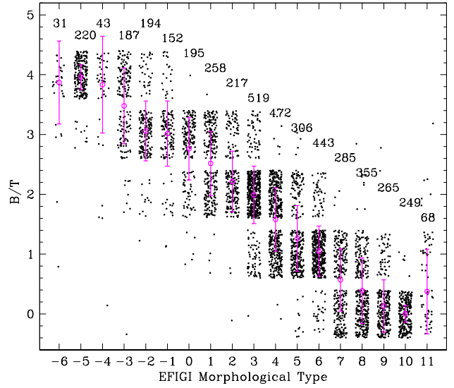
Fig. 5. Distribution of B/T versus the EFIGI morphological type for the 4458 galaxies in the EFIGI catalogue (see Table 2 for the correspondence with types). In order to see the relative density of data points, they are spread in the horizontal and vertical direction, hence the apparent rectangles. The weighted mean and weighted r.m.s. dispersion in B/T are also plotted for each type along with the corresponding number of galaxies. This graph shows the strong correlation of morphological type with B/T.
