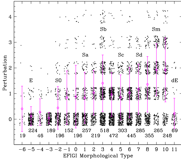
Fig. 13. Distribution of the Perturbation attribute for all 4458 EFIGI galaxies (same presentation as in Fig. 5). This graph shows the increasing Perturbation for types Sd, Sdm, Sm, and Im.
