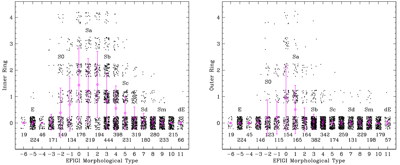
Fig. 10. Distribution of the Inner Ring (left) and Outer Ring (right) attributes as a function of EFIGI morphological type for the 3698 and 3549 EFIGI galaxies for which these attributes are defined (same presentation as in Fig. 5). Strong inner rings dominate among S0a, Sa, and Sab galaxies, whereas outer rings show a marked peak in strength for S0a galaxies only.
