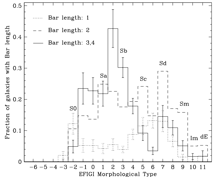
Fig. 9. Fraction of galaxies with different values of the Bar Length attribute as a function of EFIGI morphological type for the 3106 EFIGI galaxies with Inclination-Elongation \leq 2 . This graph shows that bars are frequent among all galaxy types except E and dE, and the strongest bars lie in early-type spirals. For clarity, the Poisson error bars in the fractions with Bar Length = 2 are not plotted; these are listed in Table 5 and are comparable to those for the other plotted attribute values.
