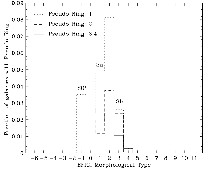
Fig. 12. Fraction of galaxies with different values of the Pseudo-Ring attribute as a function of EFIGI morphological type for the 3105 galaxies with \text{Inclination-Elongation} \leq 2 . For clarity, no error bars are plotted, as these are large due to the small number of objects (see Table 7). The outer pseudo-ring pattern is essentially present in S0 + , S0a, Sa, Sab and Sb galaxies.
