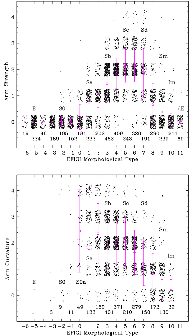
Fig. 7. Distribution of the Arm Strength (top) and Arm Curvature attributes (bottom) for the 3881 and 2127 EFIGI galaxies for which these attributes are defined (same presentation as in Fig. 5). The top panel shows the tight relation between the relative flux in the spiral arms and the morphological type, with an increase of the Arm Strength from types Sa to Sc, then a decrease from types Sd to Im. The bottom panel shows a decrease of the Arm Curvature for increasing spiral types.
