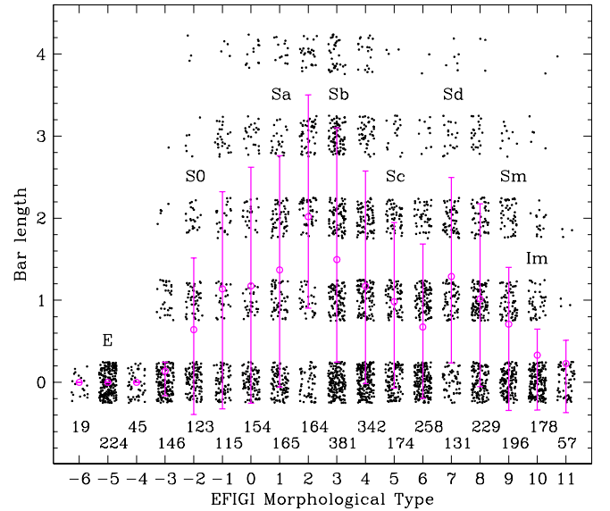
Fig. 8. Distribution of the Bar Length attribute as a function of EFIGI morphological type for the 3878 EFIGI galaxies for which this attribute is defined (same presentation as in Fig. 7). This graph shows that bars are frequent among all galaxy types except for the cE, E, cD, and dE galaxies, and the strongest bars lie in early-type spirals.
