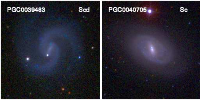
Fig. 17. “True colour” irg images of the two dwarf spiral galaxies found in the EFIGI catalogue. These galaxies have redshifts 0.0026385 and 0.0006414, absolute g magnitudes of -16.9 and -14.8 , and intrinsic D_{25} values of 5.7 kpc and 1.9 kpc.
