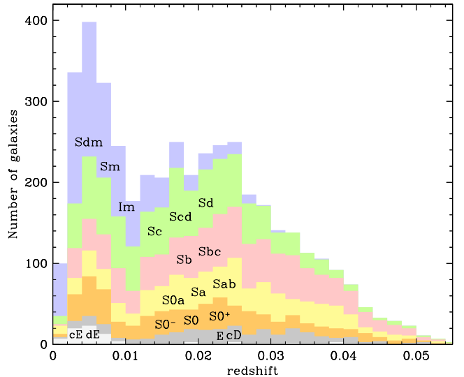
Fig. 1. Redshift distribution of all EFIGI galaxies separated by EFIGI morphological type, grouped as follows: cE-dE (light grey) ; E-cD (grey); S0 - -S0-S0 + (orange); S0a-Sa-Sab (yellow); Sb-Sbc (pink); Sc-Scd-Sd (green); Sdm-Sm-Im (blue).
