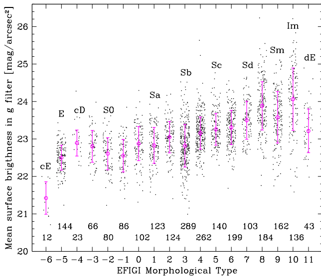
Fig. 18. Distribution of mean surface brightness in the g -band within the D_{25} diameter for the 2278 EFIGI galaxies with \text{Inclination-Elongation} \leq 2 and \text{Contamination} \leq 1 as a function of EFIGI morphological type. For each type, the weighted mean and r.m.s. dispersion (with 3-sigma clipping) are also plotted as a circle and vertical error-bar. The mean surface brightness is decreasing along the Hubble sequence from cE to Im types.
