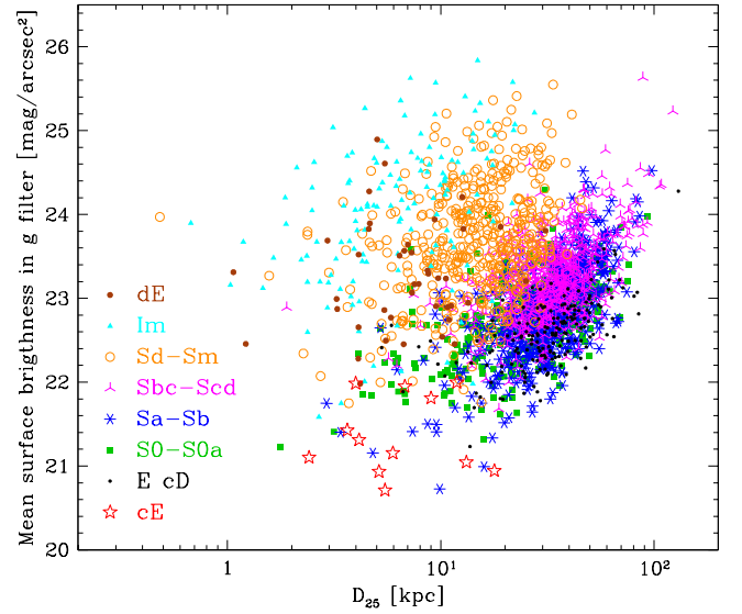
Fig. 19. Distribution of apparent major isophotal diameter D_{25} converted into kpc as a function of mean surface brightness in the g -band within the D_{25} diameter for the 2278 EFIGI galaxies for which these parameters are defined and with \text{Inclination-Elongation} \leq 2 and \text{Contamination} \leq 1 . Different symbols are used for different EM-types. This graph shows that galaxies with a surface brightness of dE but a more extended diameter could be detected in the EFIGI catalogue.
