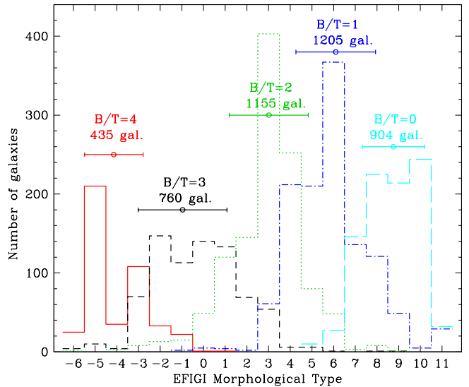
Fig. 6. Histograms of EFIGI morphological type for the five values of B/T (decreasing from left to right). The weighted mean and r.m.s. dispersion in the morphological type are plotted above each histogram along with the corresponding number of galaxies. This graph shows the large dispersion in morphological type for a given B/T.
